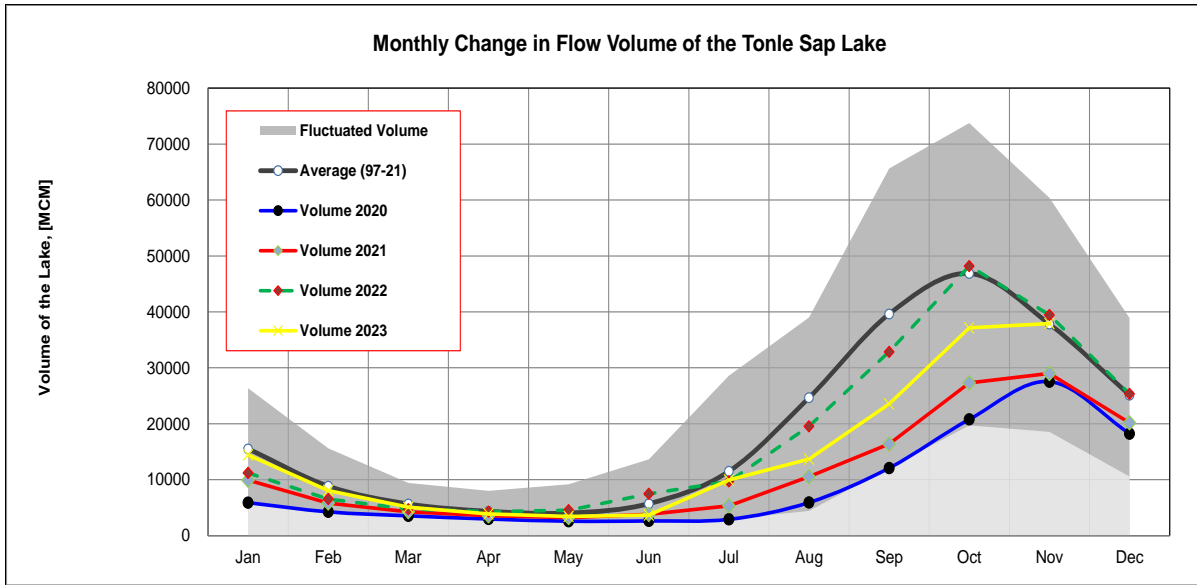
Figure 13. The seasonal change in monthly flow volume of Tonle Sap Lake.
